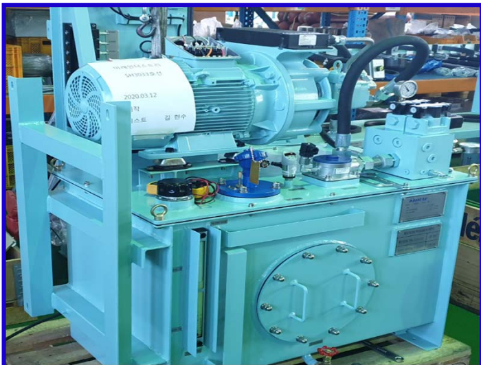
WINCH CONTROL HYDRAULIC POWER UNIT
