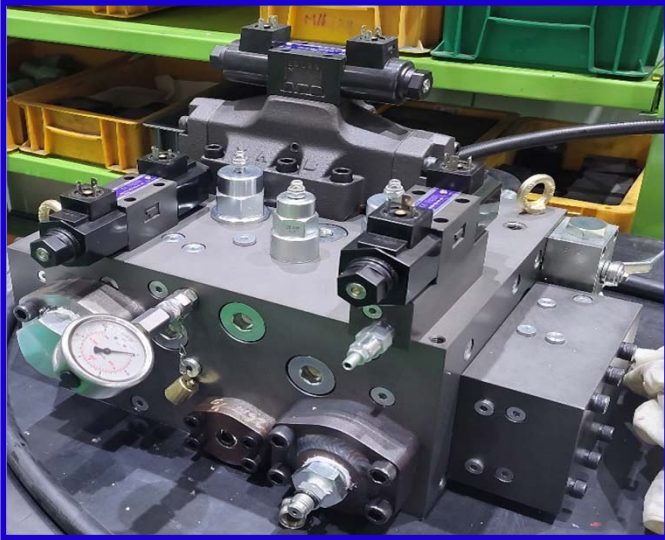
MANIFOLD BLOCK FOR SHIP YARD
